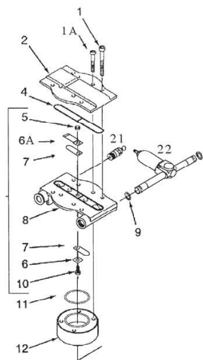
(FIG 1) FOR MODELS 71R545-P315B COVER/VALVE PLATE ASSM. SHOWN SEPARATELY TO SHOW HIGH PRESSURE END OF UNIT
