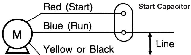
< MOTOR WITH 3 LEADS & CAPACITOR
