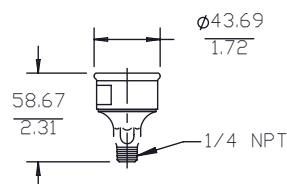
MUFFLER ASM. - UNATTACHED
