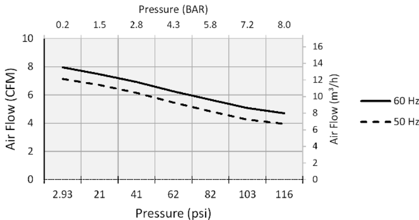
120R-40BQ3 Air Flow
