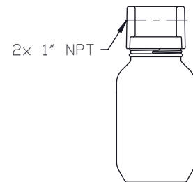
FILTER ASM.
