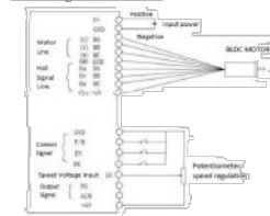
Connection Diagram of motor and driver
