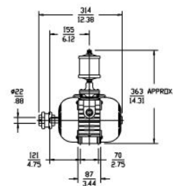
VIEW LESS MUFFLER
