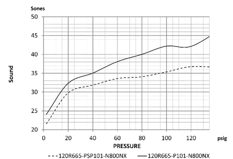
SOUND LEVEL @ PRESSURE
